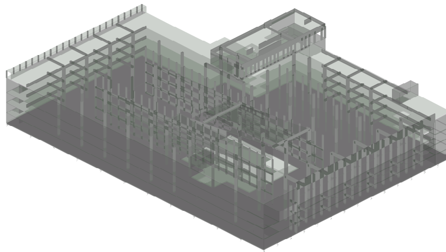
GARAGE – 3D MODEL
