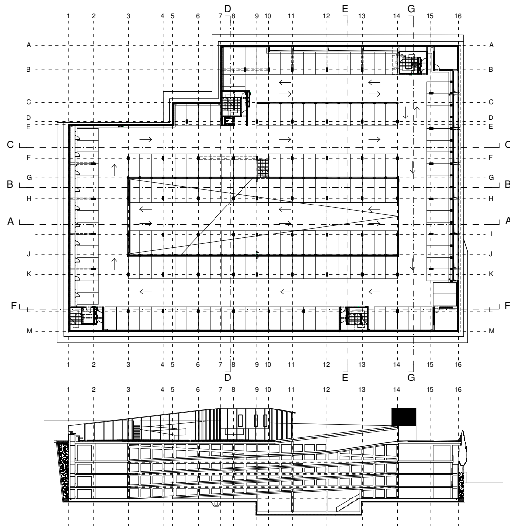
PLAN OF GROUND FLOOR -1 AND SECTION A-A
